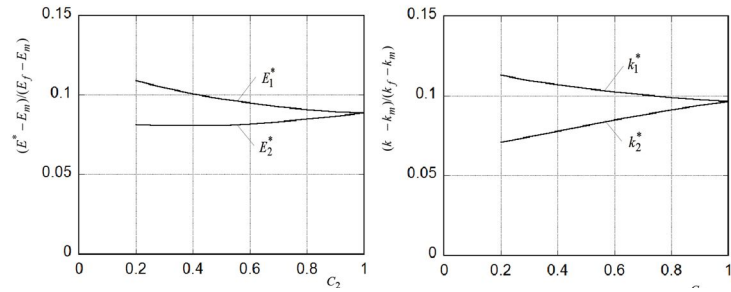
Fig. 3 A model of a composite material Fig. 4 Effective Young's Moduli E^* and thermal conductivities k^* under contact and Joule heating.
