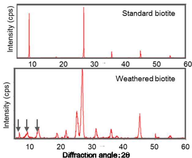
Fig.1 Powder X-ray Diffraction patterns of biotite
