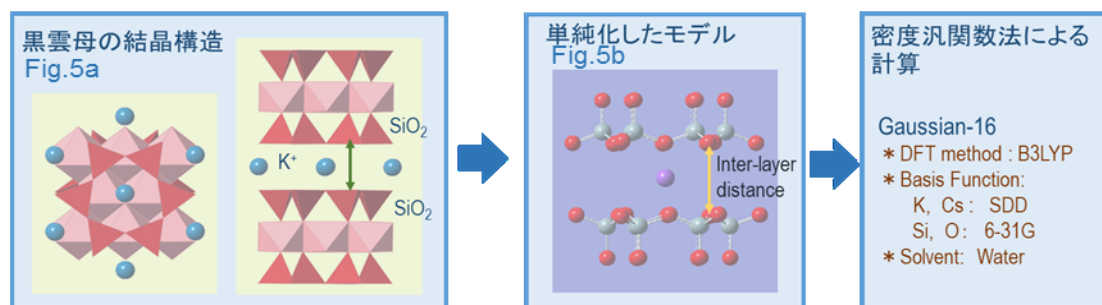
Fig.5 Quantum chemical simulation model of weathered biotite
