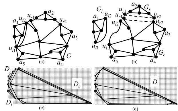
Fig. 1 (a) Plane graph G , (b) subgraphs G_l , G_r and G_c , (c) convex grid drawings D_l of G_l , D_r of G_r , and D_c of G_c , and (d) convex grid drawing D of G .
