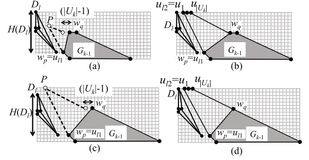
Fig. 10 Illustrations for (a),(b) Case (i), and (c),(d) Case (ii).
