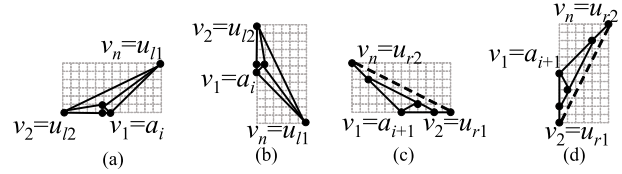
Fig. 9 (a) A triangular drawing of G_l , (b) a drawing D_l of G_l , (c) a triangular drawing of G_r , and (d) a drawing D_r of G_r .
