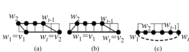
Fig. 5 Drawings D_1 of G_1 (a), (b) for Case 1 and (c) for Case 2.
