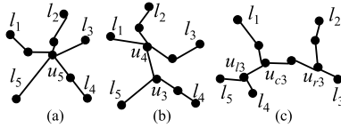
Fig. 8 Decomposition trees T(G) (a) having a node of degree five, (b) having a node of degree four and a node of degree three, and (c) having three nodes of degree three.
