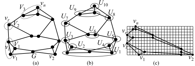
Fig. 4 (a) An internally triconnected plane graph G , (b) a canonical decomposition \Pi of G , and (c) a pentagonal drawing of G .
