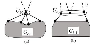
Fig. 3 (a) Graphs G_k for which |U_k| = 1 and (b) |U_k| \geq 2 .
