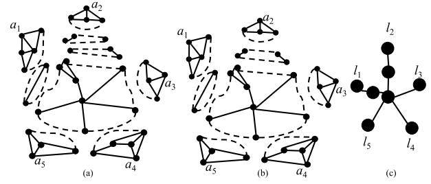
Fig. 2 (a) Split components of the graph G in Fig. 1(a), (b) triconnected components of G , and (c) a decomposition tree T(G) .
