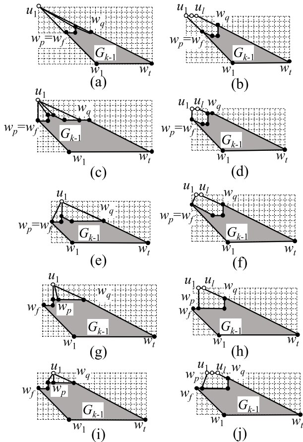
Fig. 7 Installing U_k to D_{k-1} .
